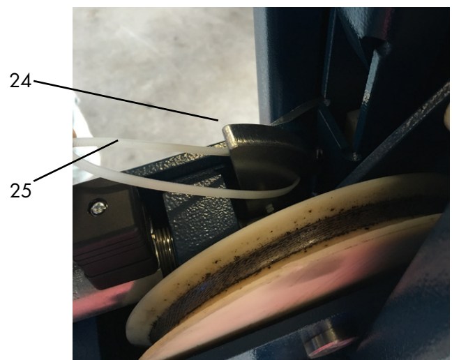
24 Safety catches 012 25 cable ties/wire
